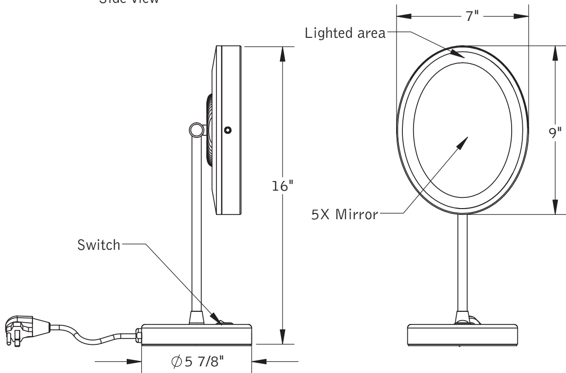
Side view
